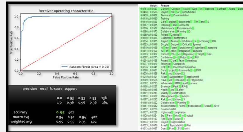
Predict project performance using ML
